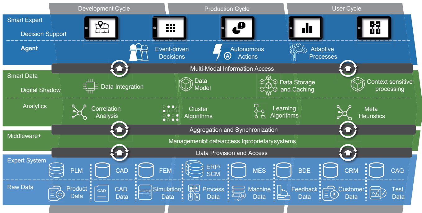
Infrastructure of the Internet of Production – IoP
